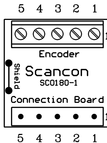
Pin Header – Connection Board
