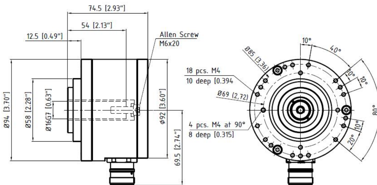
SCH94L M23 connector
