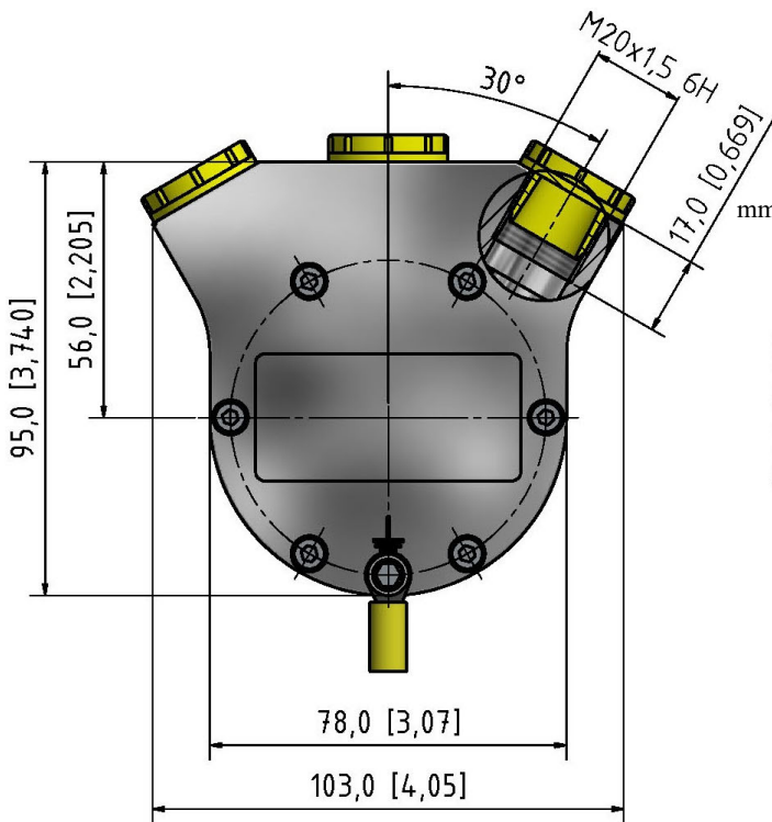
Side Standard End Cap (FE)
