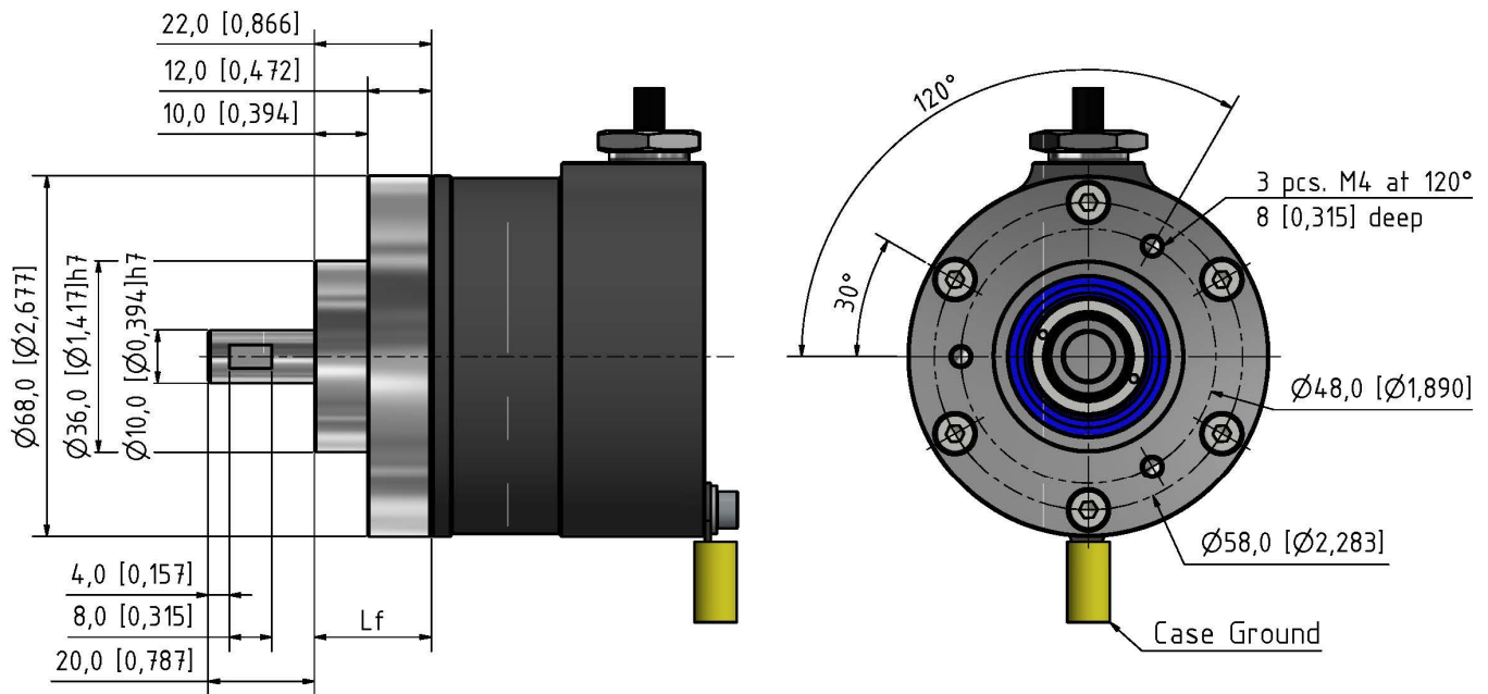
Face Mount K
