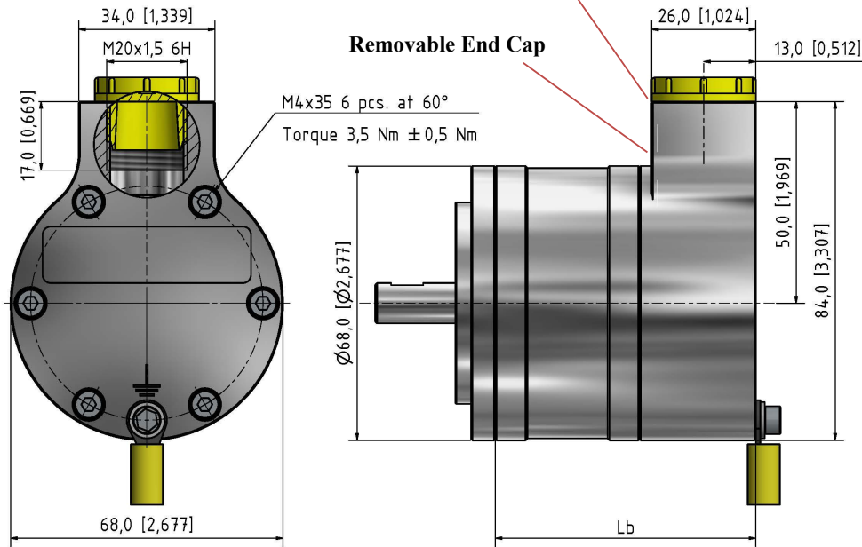
Removable End Cap Side Standard (EC01)
